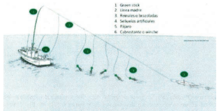
Figura 1. Ilustración de un green stick. Fuente: modificado de Bailey Farnsworth/The Pew Charitable Trusts ( http://safinacenter.org/2016/06/fishing-gear-101-greenstick-gear-buoygear-innovative-way-fish-tuna-swordfish/ ).
